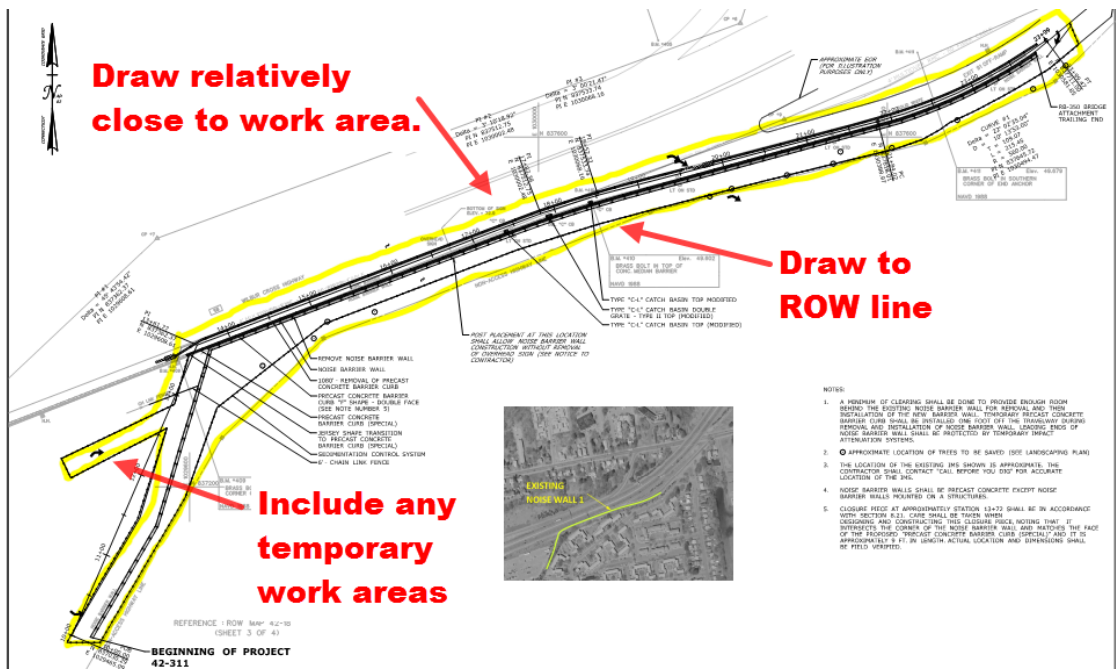
Figure 230 - Highway Project without Full Depth Reconstruction
