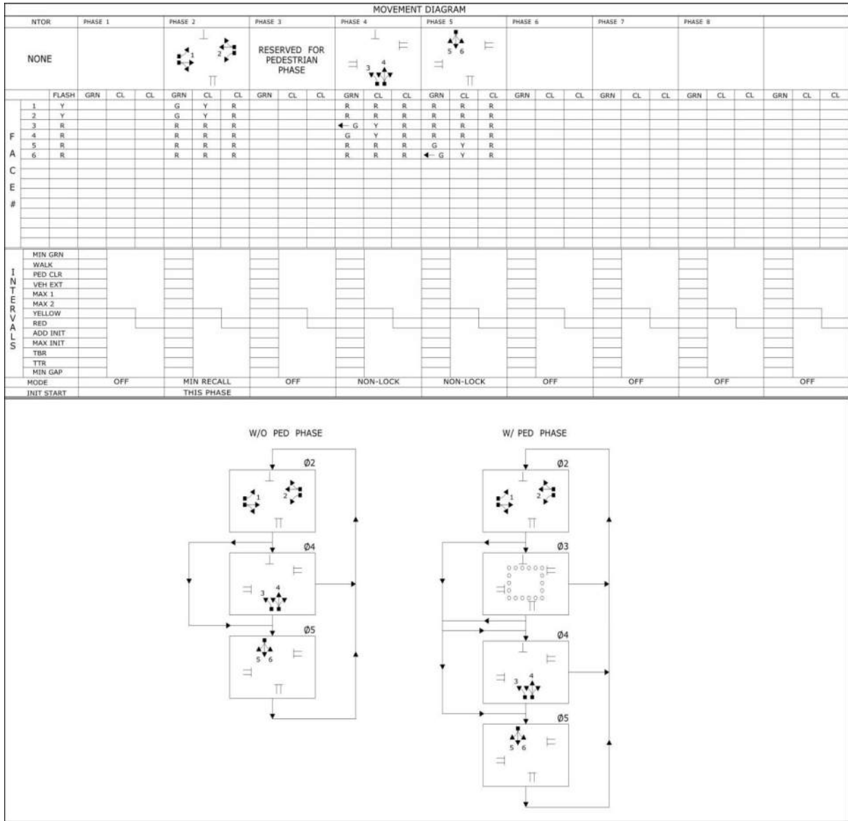
Figure 4-8 Split Phasing
