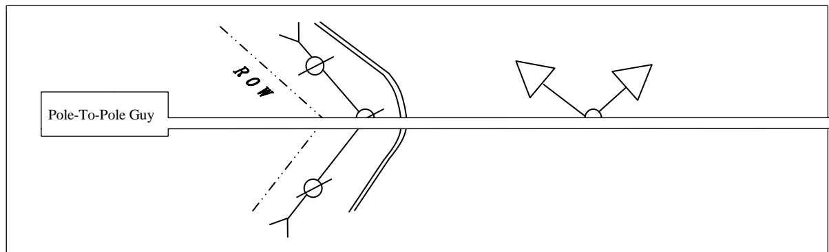
Figure 15-9 Pole-To-Pole Guy
