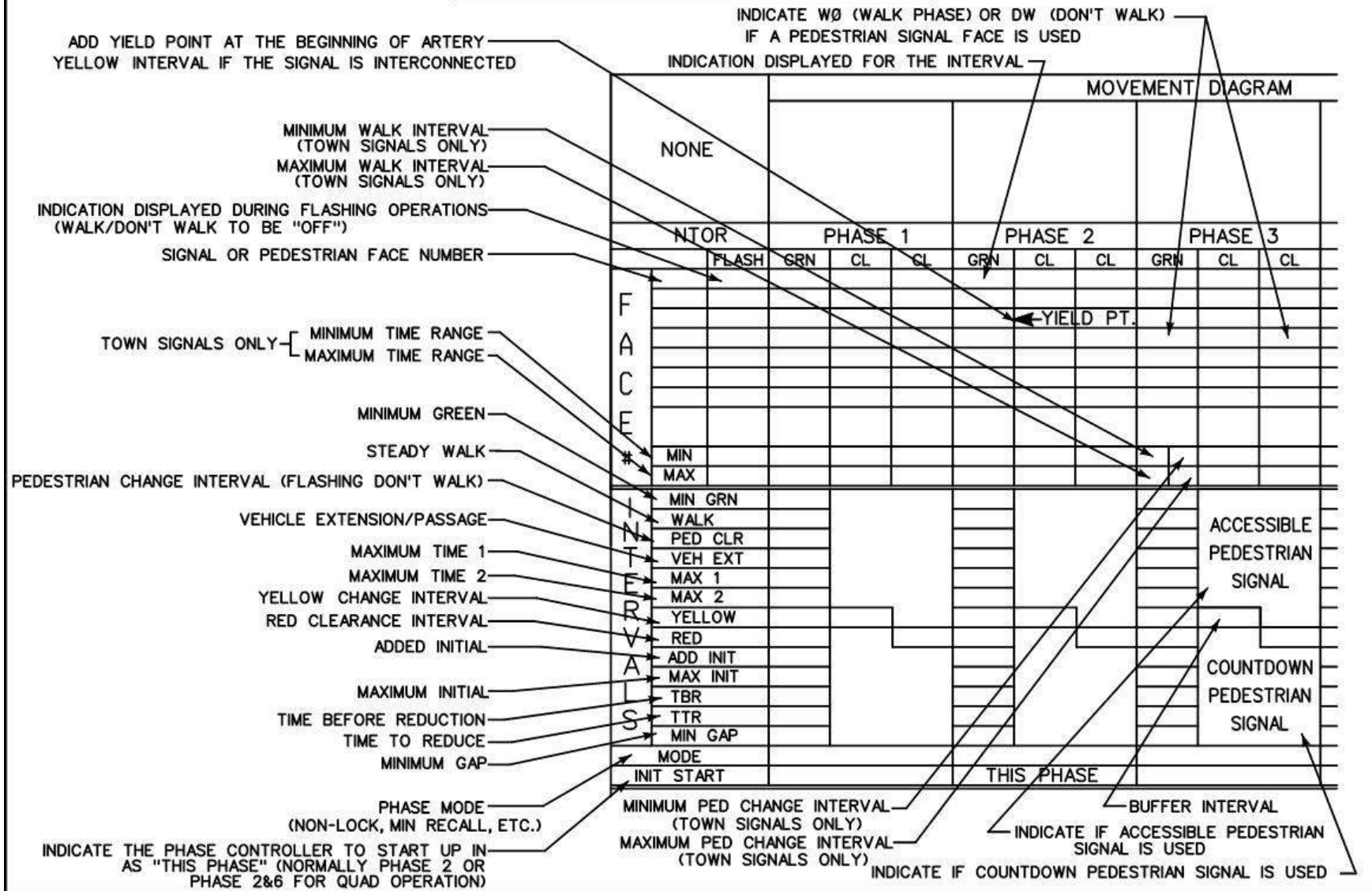
Figure 16-2 Sequence and Timings
