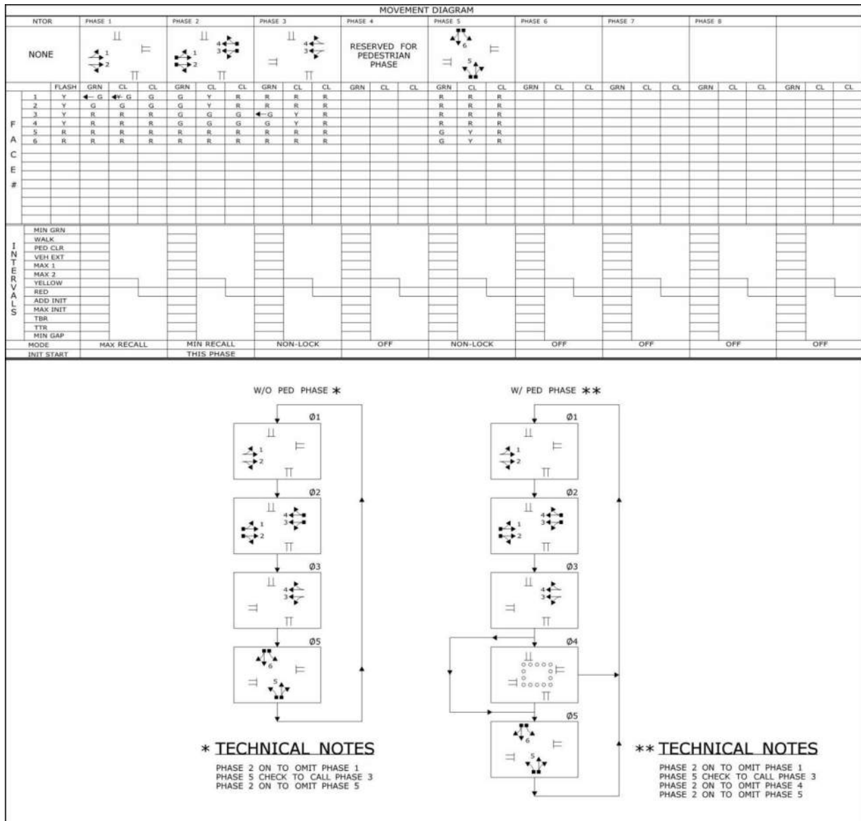
Figure 4-12 Lead-Lag (Protected-Permitted)
