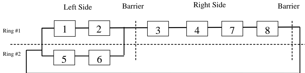
Figure 4-2 NEMA Dual Ring, Quad/Sequential Diagram
