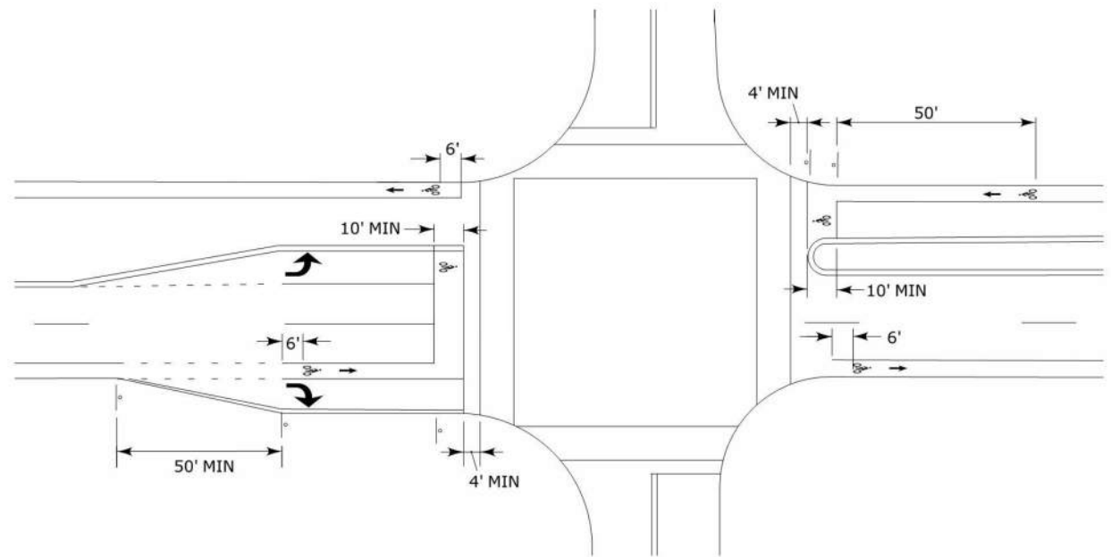
Figure 7-6 Bicycle Box
