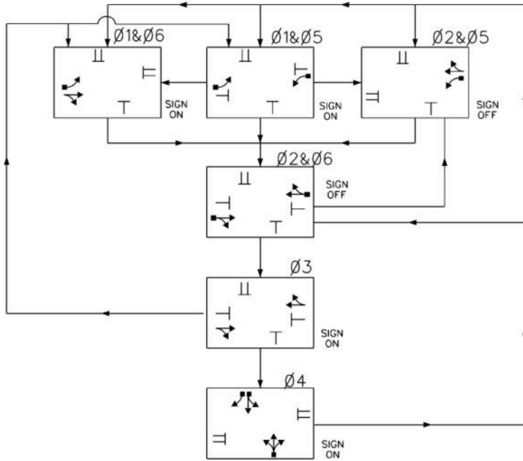
Figure 14-4 Quad Phasing with Sign on one Artery Approach
