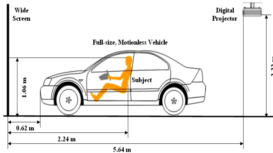
Figure 21 Schematic diagram of lab setup
