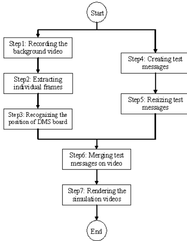
Figure 18 Flowchart for the simulation video development
