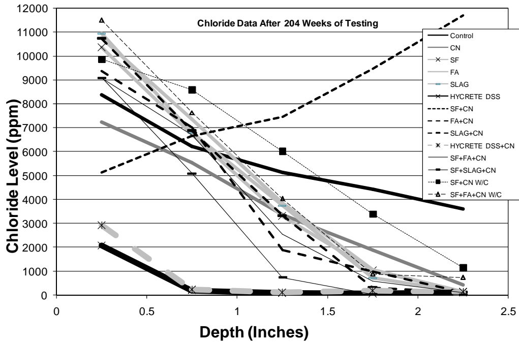
Figure 5.3: Chloride Level Versus Depth (VTrans Results)
