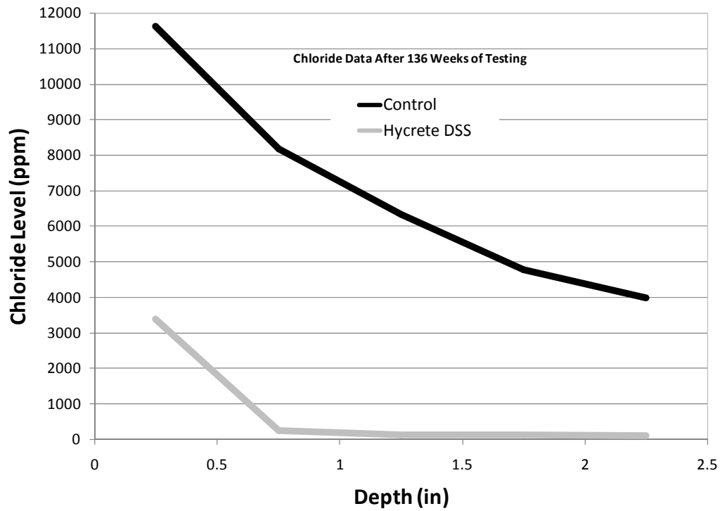
Figure 5.4: Chloride Level Versus Depth (Grace Results)
