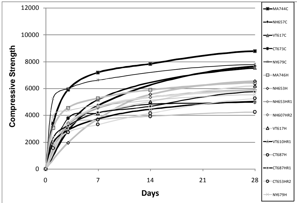
b) 0 to 28 Day Strengths
