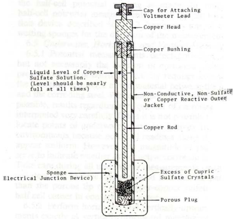
Figure 2.2: Copper-Copper Sulfate Half Cell Circuitry (ASTM 1999)
