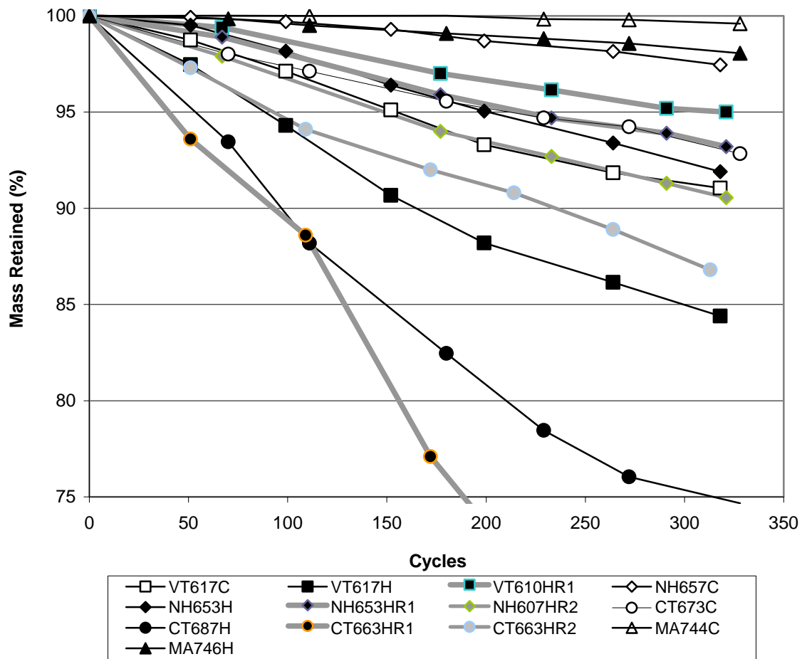
Figure 5.5: Percent Mass Loss of Specimens in Freeze Thaw Test Protocol
