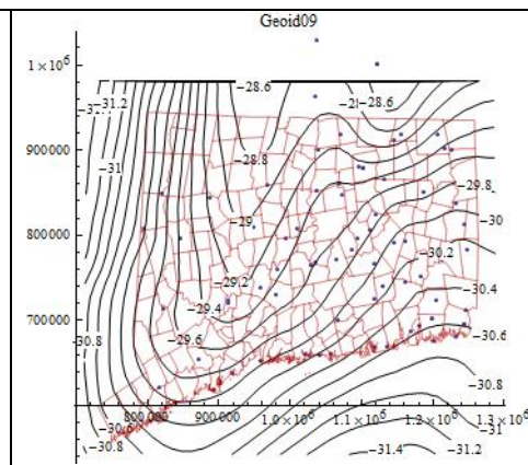
Figure 2. GEOID09 geoid heights (m). Dots indicate observed stations.
