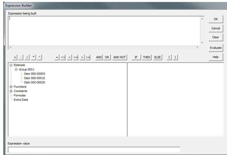
Figure 4-16. Expression Builder Window
