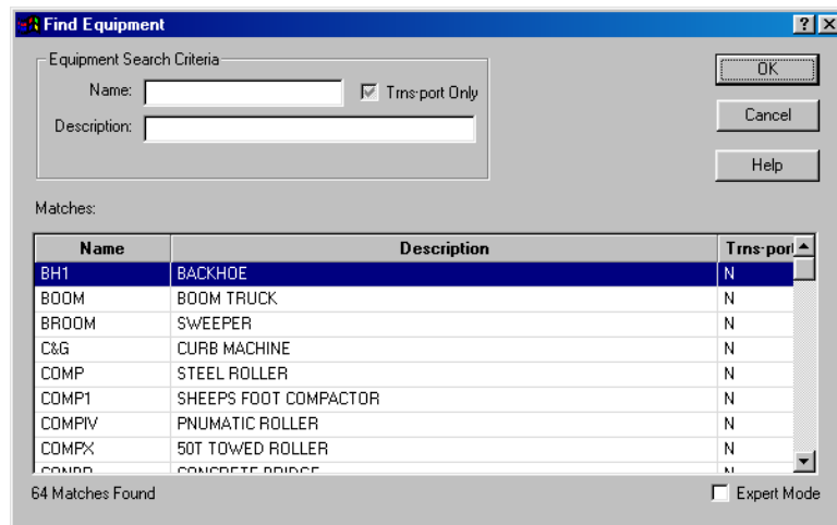
Figure 5-23. Find Window
