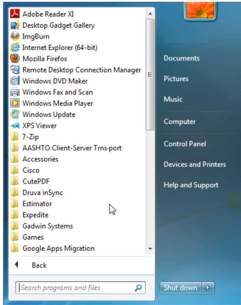
Figure 4-1. Starting Estimator
