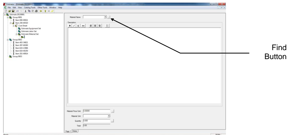
Figure 5-22. Find Button
