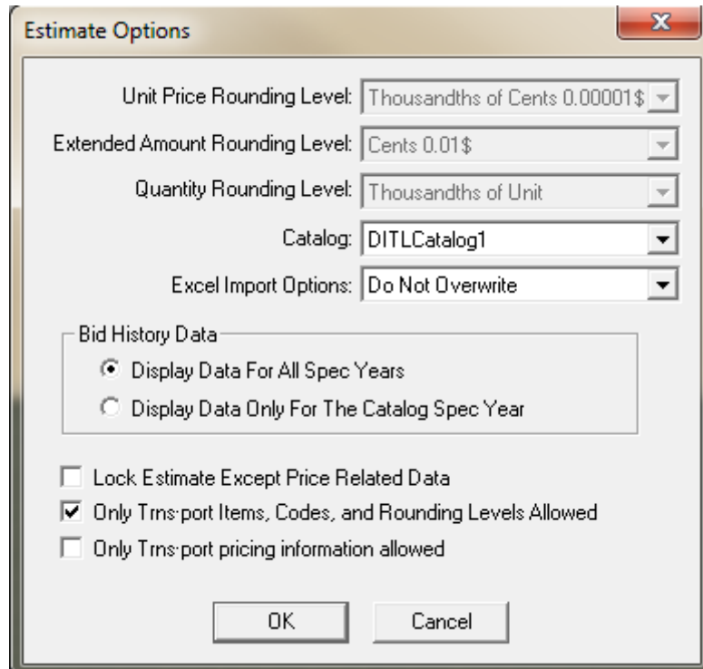
Figure 8-6. Estimate Options
