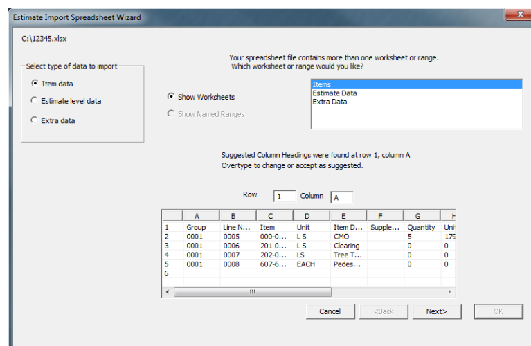
Figure 8-7. Estimate Import Spreadsheet Wizard – Importing Item-Level Data
