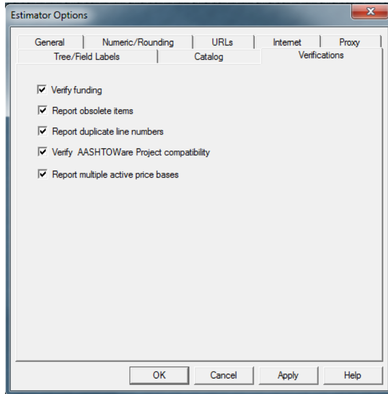
Figure 4-14. Global Options Window - Verifications Tab
