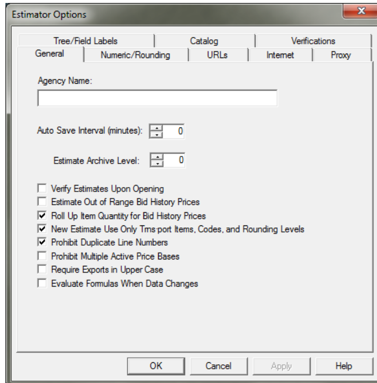
Figure 2-10. The Global Options Window – General Tab
