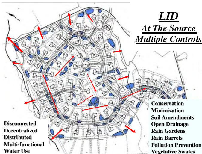
Figure 6.2.2 – LID Controls. A LID approach use a wide array of techniques that work with the landscape, soils, drainage patterns and vegetation to minimize impacts and integrated management controls to retain, detain, infiltrate and filter runoff. LID can provide better stormwater controls by mimicking the pre-development hydrology. Often LID designs increase lot yield and reduce infrastructure cost.
