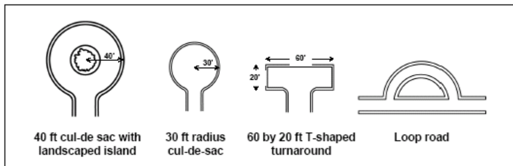
Figure 6.4.9 – Different styles of turnarounds. Source: Adapted from Atlanta Regional Commission, 2001.
