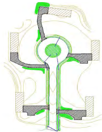
Figure 6.3.7 – Cul-de-sac designs.
