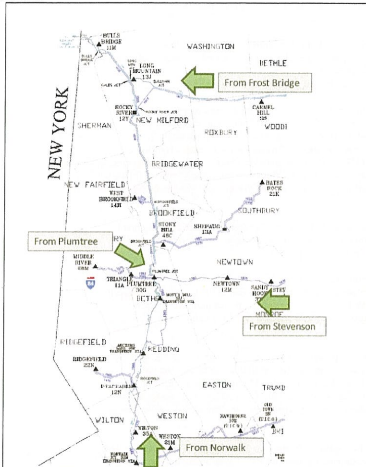
The above diagram shows transmission connections to the HV sub-area load pocket (green arrows). 115-kV connections are shown in violet, 345-kV connections are shown in blue. (Eversource 1, Vol. 1, p. 2-12, Vol. 4, Fig. 5-2)
