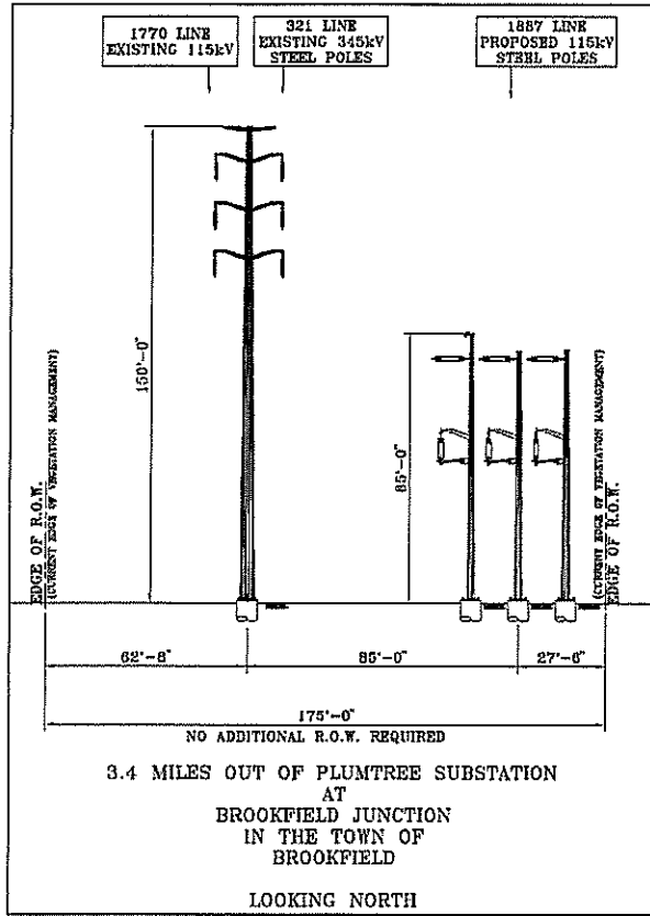
Figure 3: Cross section of the existing right-of-way with the new transmission line at Brookfield Junction.
