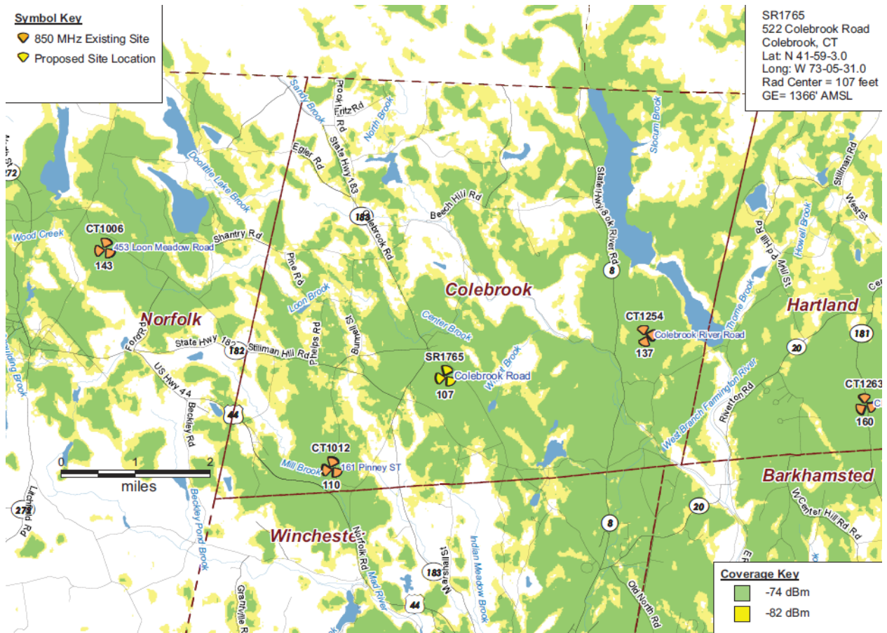
Figure 8: Existing and Proposed Coverage at Antenna Height of 107 feet
