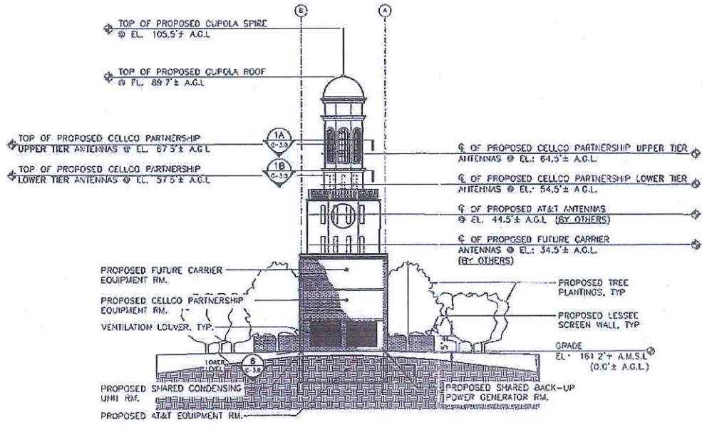
2 EAST ELEVATION C-4.0 SCALE: 1" = 20'
