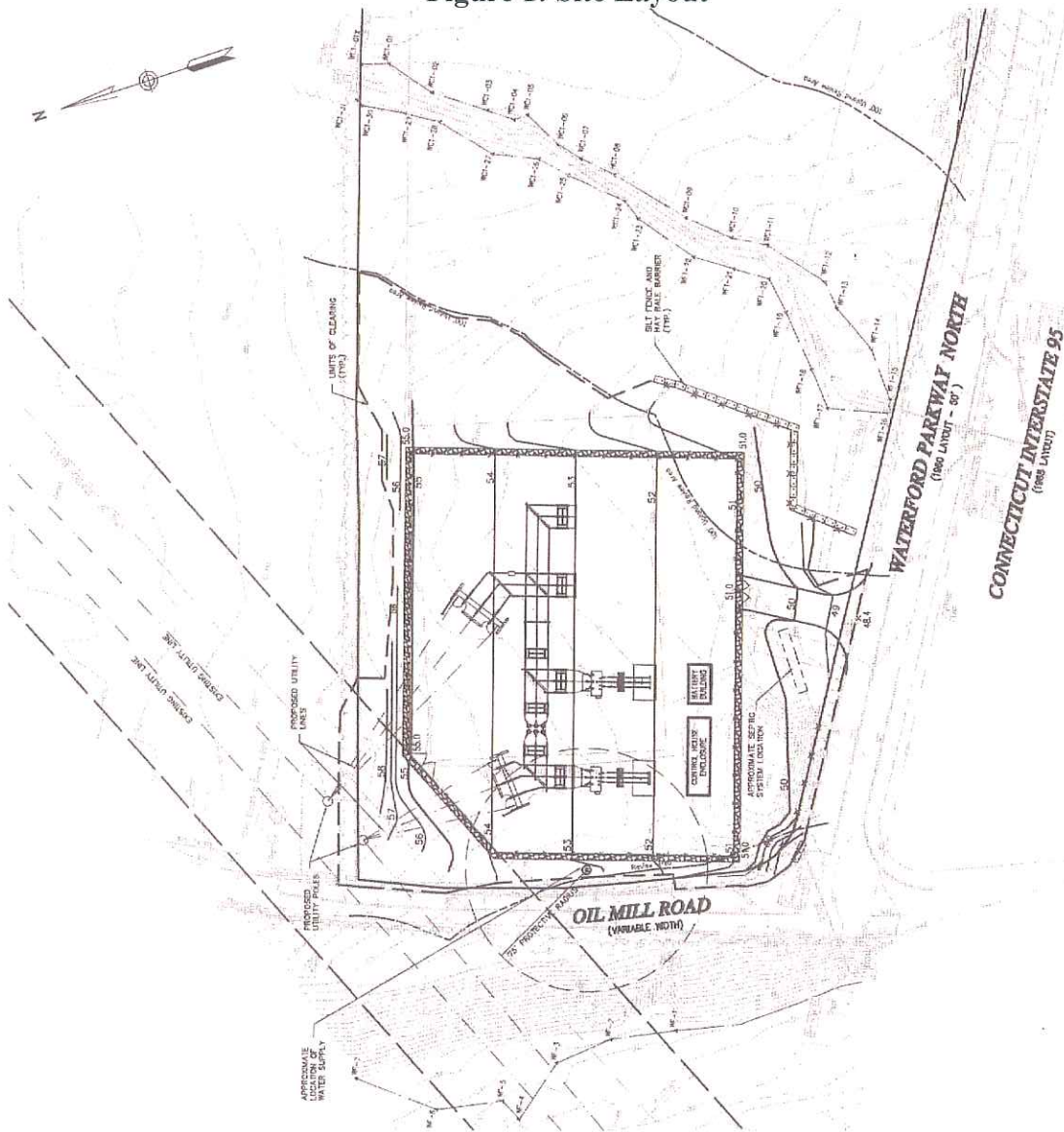
Figure 1: Site Layout
