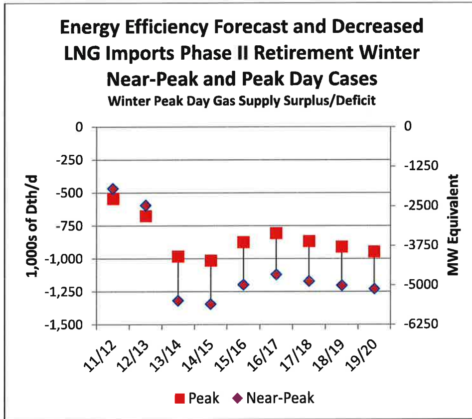
Exhibit B-123. Comparison of Energy Efficiency Forecast and Decreased LNG Imports Phase II Retirement Winter Near-Peak and Peak Day Case Results
