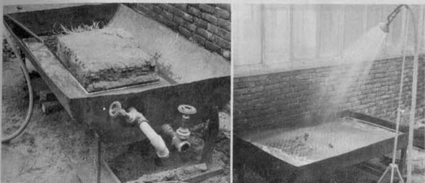
FIGURES 10 and 11. A soil monolith with oat plants on the pin-board rests in the washing tank as it is filled with water for soaking. During washing the tank are adjusted to lower the water level as soil is washed away.
