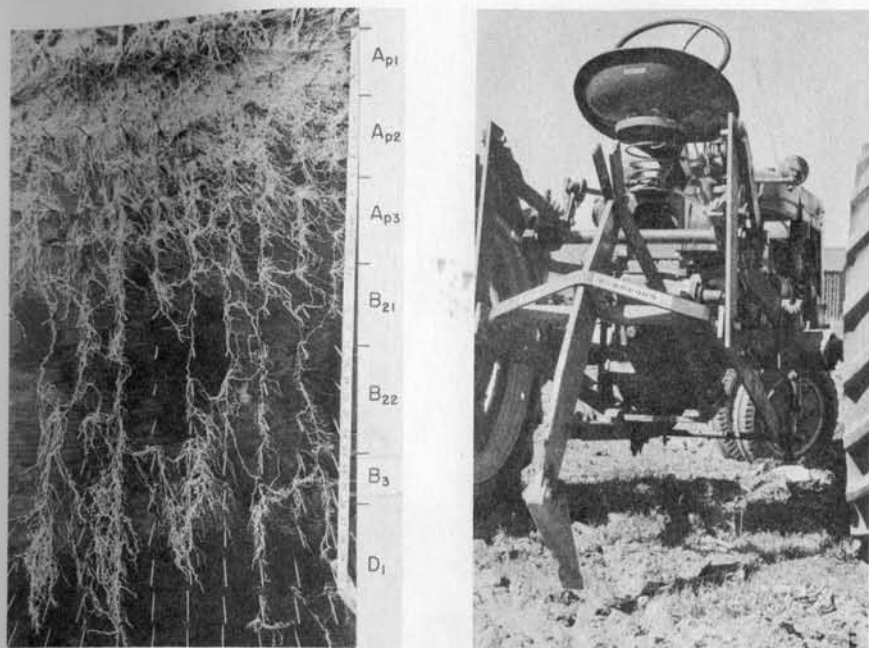
FIGURE 16. Roots of rye 33 weeks old taken from the profile shown in Figure 14 and described on page 11. Root growth is noticeably less dense in the compaction zone; roots passing through are well branched in deeper subsoil ( B_3 ) and substratum ( D_1 ).
