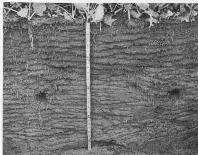
FIGURE 20. Profile of Merrimac sandy loam with compaction pan at about 9 or 10 inches, mainly the B_{21} horizon. Shown about 10 weeks after the soil was chiseled and then seeded with rape in early September.
