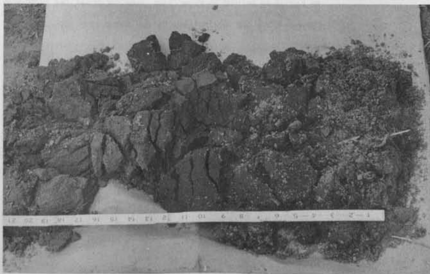
FIGURE 3b. The compaction pan (9 to 17 inches) shown in Figure 3a forms a laminated layer. The blocklike clods were fractured by hand into weak platy fragments, coarse to very coarse, on surfaces of weakness.
