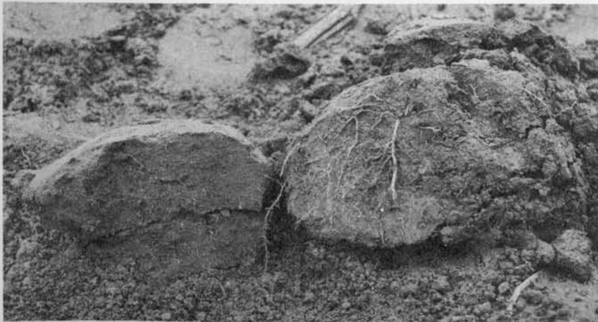
FIGURE 4b. The furrow slice and compaction pan clods shown in Figure 4a turned to show their common plane, the plow sole. Roots grew to the bottom of the plowed layer at right, then turned along the distinct top of the compacted soil at left.
