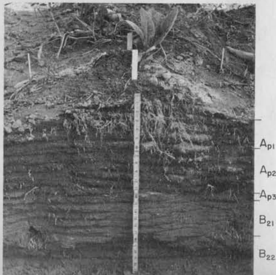
FIGURE 23. Merrimac sandy loam profile on a harvested tobacco plot, one year after being subsoiled. Subsoiler channels at 16- to 17-inch depth between the rows are clearly defined and filled with tobacco roots.
