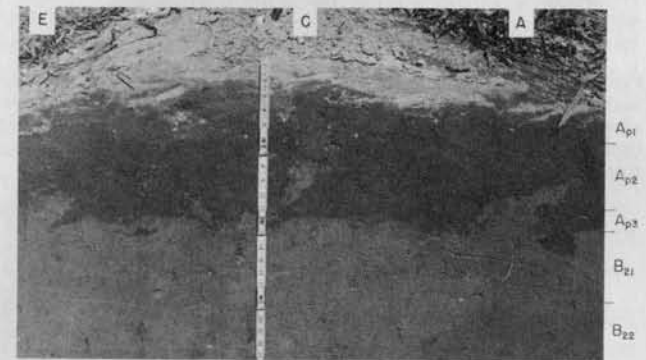
FIGURE 25. Merrimac sandy loam profile across a row of harvested tobacco. The plot was loosened and fertilized to a depth of 16 inches at the time of 8- to 9-inch spring plowing. Light-colored subsoil ( B_{21} material) has been lifted into the A_p horizon. At A, C, and E the subsoiler used with a 16-inch plow left its mark in the A_{p2} and A_{p3} horizons.
