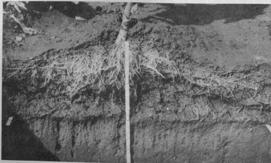
FIGURE 2. The 6-inch section here washed away from the soil profile dug across the tobacco row shows this pattern of the Havana Seed tobacco root system. Roots are largely confined to the upper 6 inches; the compaction pan, shown protruding, stopped root penetration. Wires thrust into the profile help to hold roots in position.
