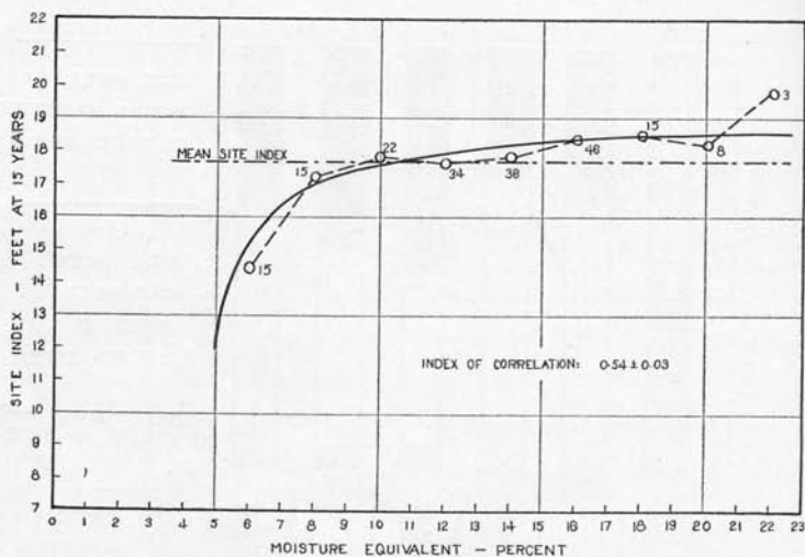
FIGURE 62. The relation of site index to moisture equivalent of the A_{1-2} horizon. Basis, 194 plots.
