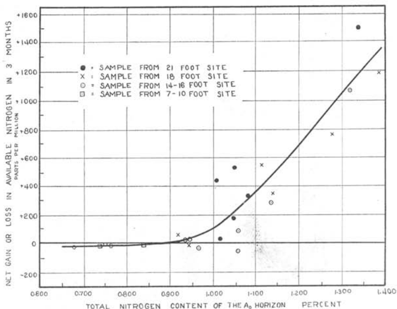
FIGURE 67. The relation of the total nitrogen content of the A_0 horizon to the changes in available nitrogen (both ammonia and nitrates) during three months of incubation.
