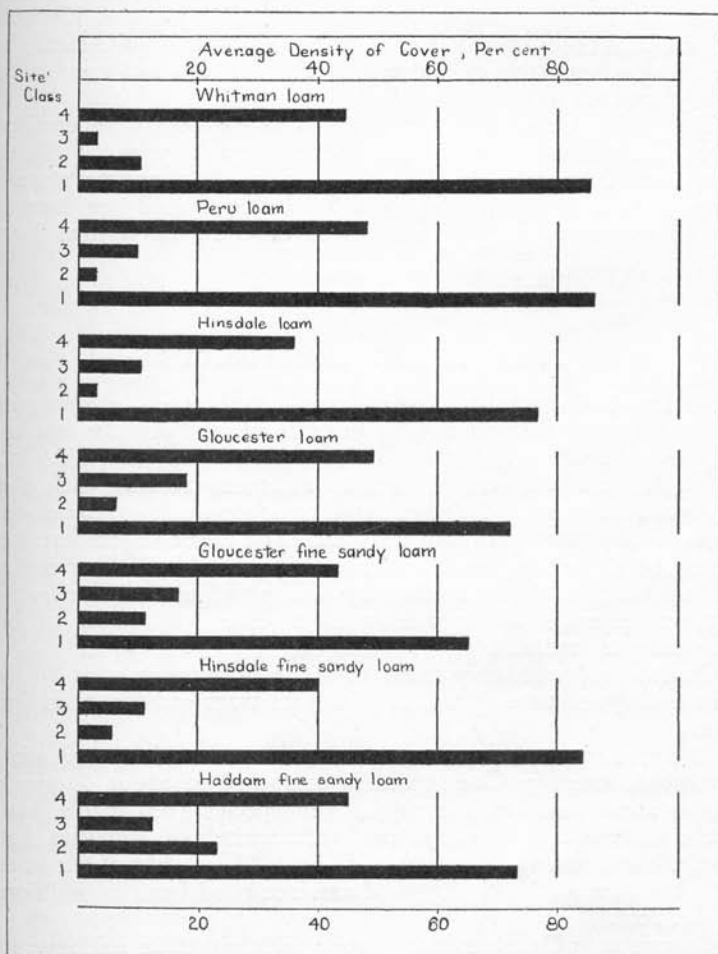
FIGURE 57. Showing average density of cover in the various vegetational layers on seven soil types.
