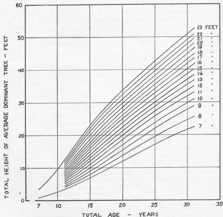
FIGURE 58. Polymorphic site index curves for planted red pine. Plotted from Table 18. Classification age, 15 years. Based on the measurement of more than 2,000 trees.
