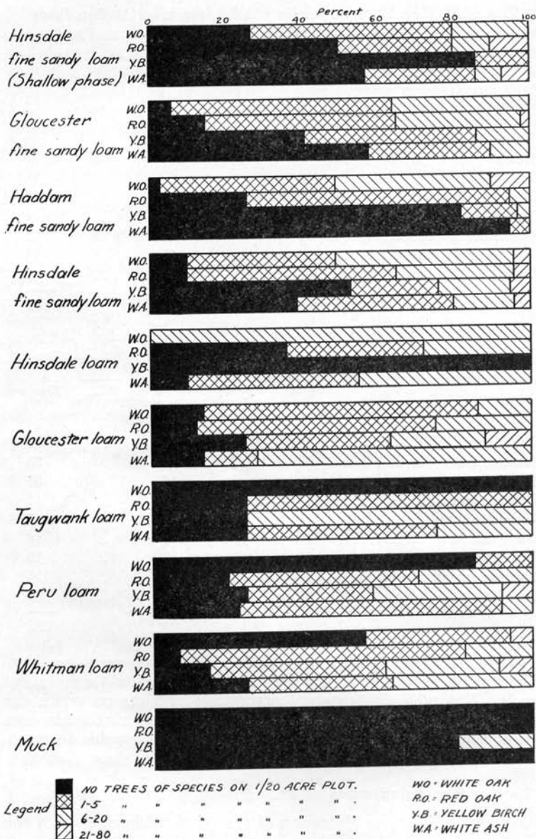
FIGURE 54. The distribution of white oak, red oak, yellow birch, and white ash on 10 soil types according to the number of trees per 1/20 acre plot. Data from Tables 10, 11, 12 and 13.
