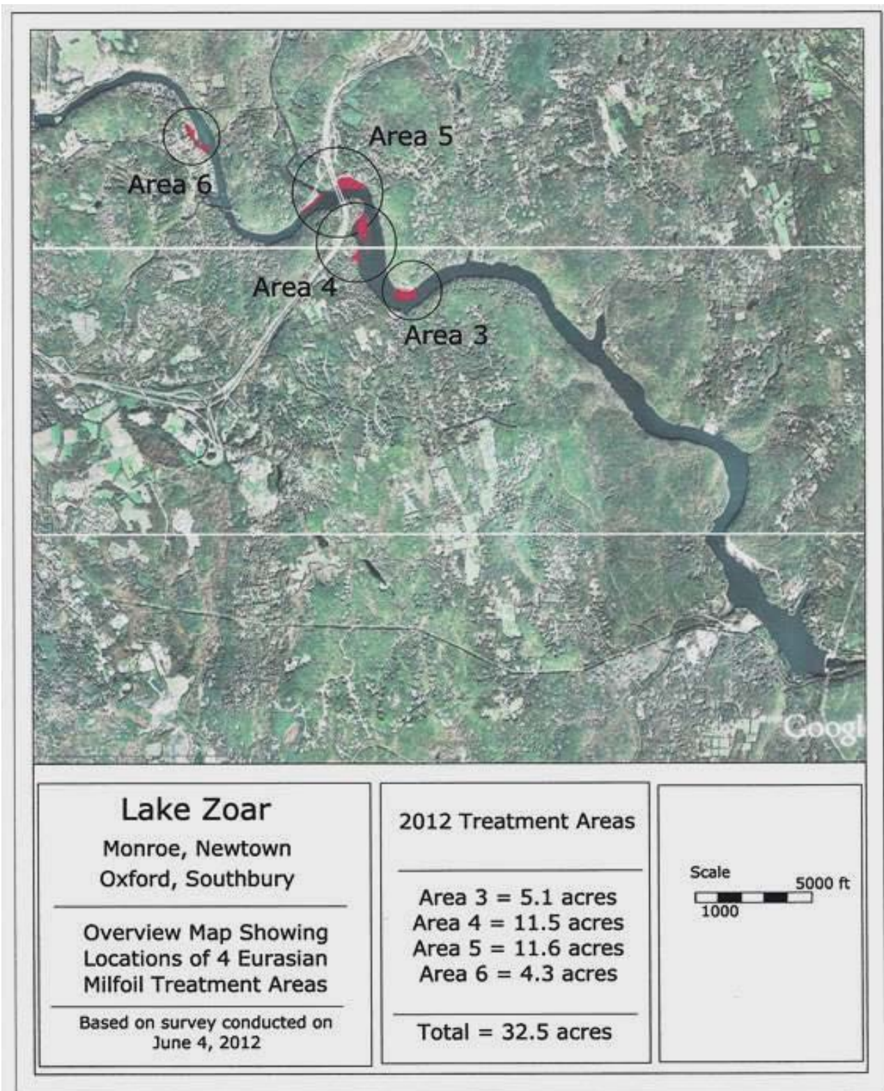
Figure 14. Locations of herbicide treatments to Lake Zoar in 2012 (Knoecklein 2012).
