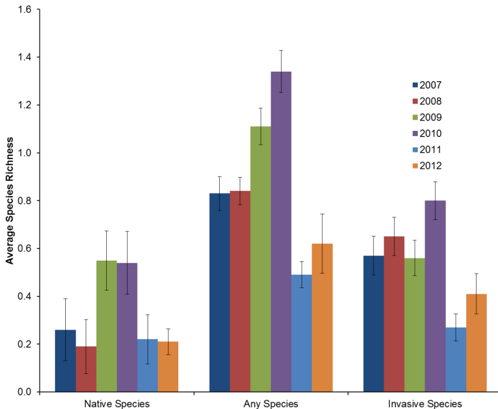
Figure 17. Yearly comparisons of average number of species per transect point in Lake Zoar. Error bars equal +/- one standard error of the mean.
