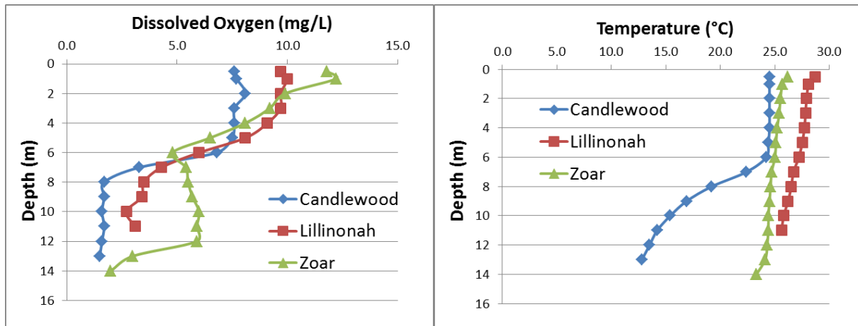
Figure 18. Temperature and dissolved oxygen profiles in Lakes Candlewood, Lillinonah, and Zoar.
