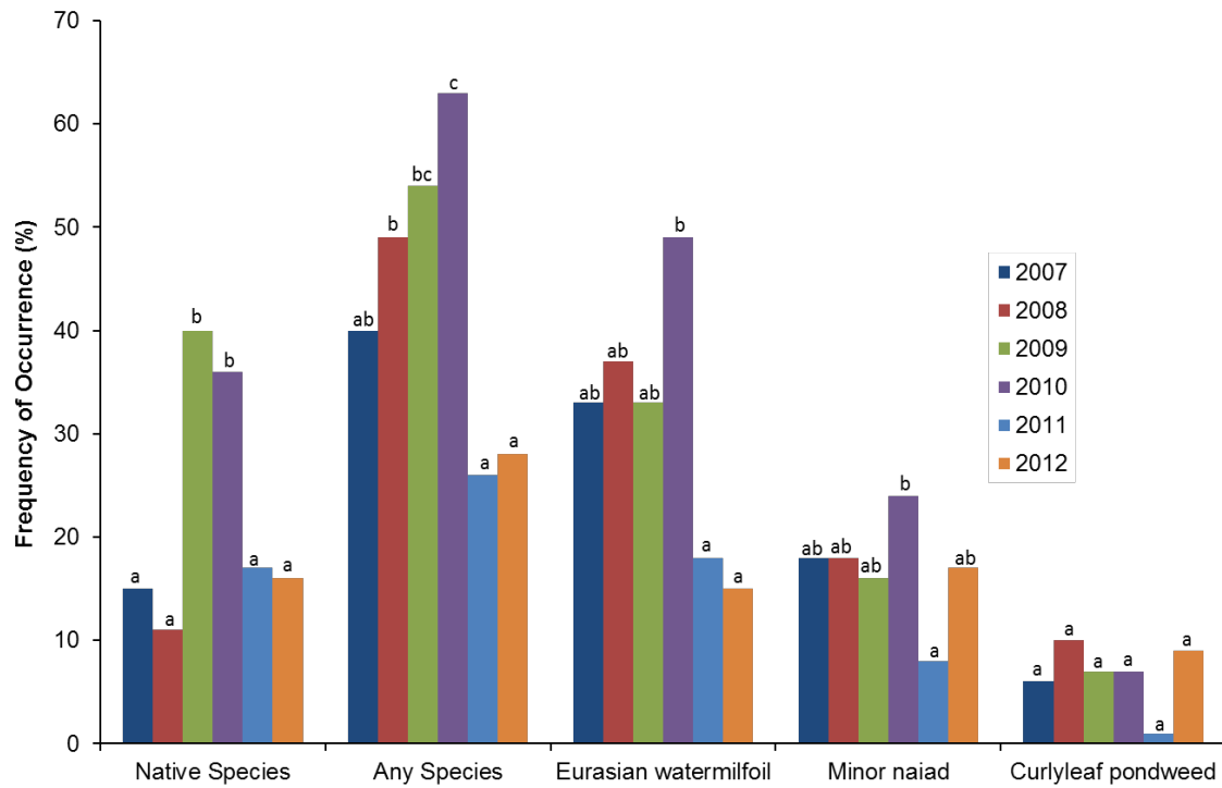
Figure 16. Yearly comparison of average frequency of occurrence of aquatic plants on transects in Lake Zoar. Bars with the same letter within a species are not statistically different.
