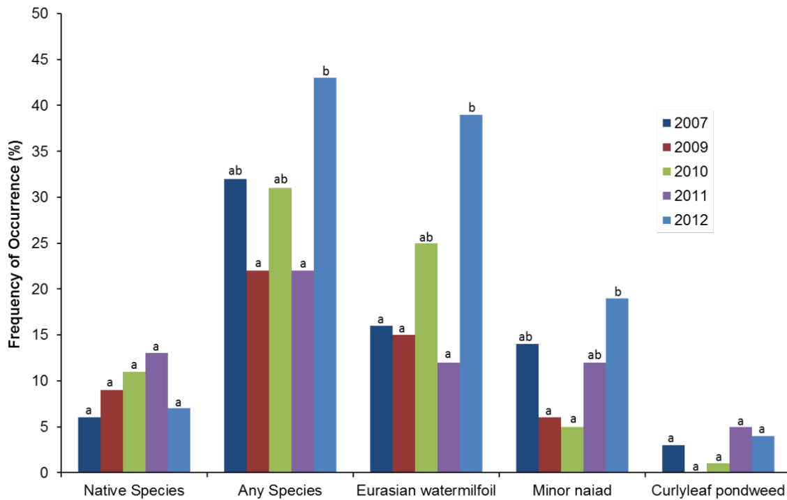
Figure 11. Yearly comparisons of the frequency of native and invasive plants on transects in Lake Lillinonah. Bars with the same letter are not significantly different.
