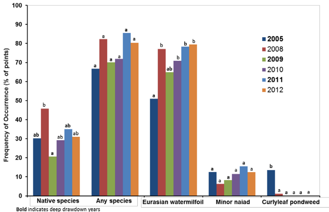
Figure 4. Yearly frequency of occurrence of aquatic vegetation on transects in Candlewood Lake. Bars with the same letter within a species are not statistically different.
