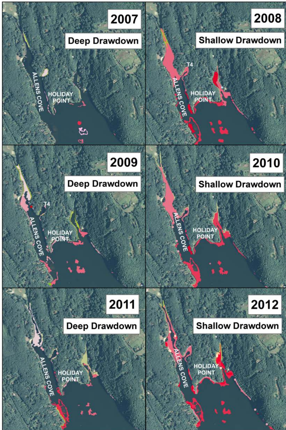
Figure 7. Comparison of the coverage and abundance of Eurasian watermilfoil in Allen's Cove from 2007 to 2012. Darker pink colors indicate greater abundance.
