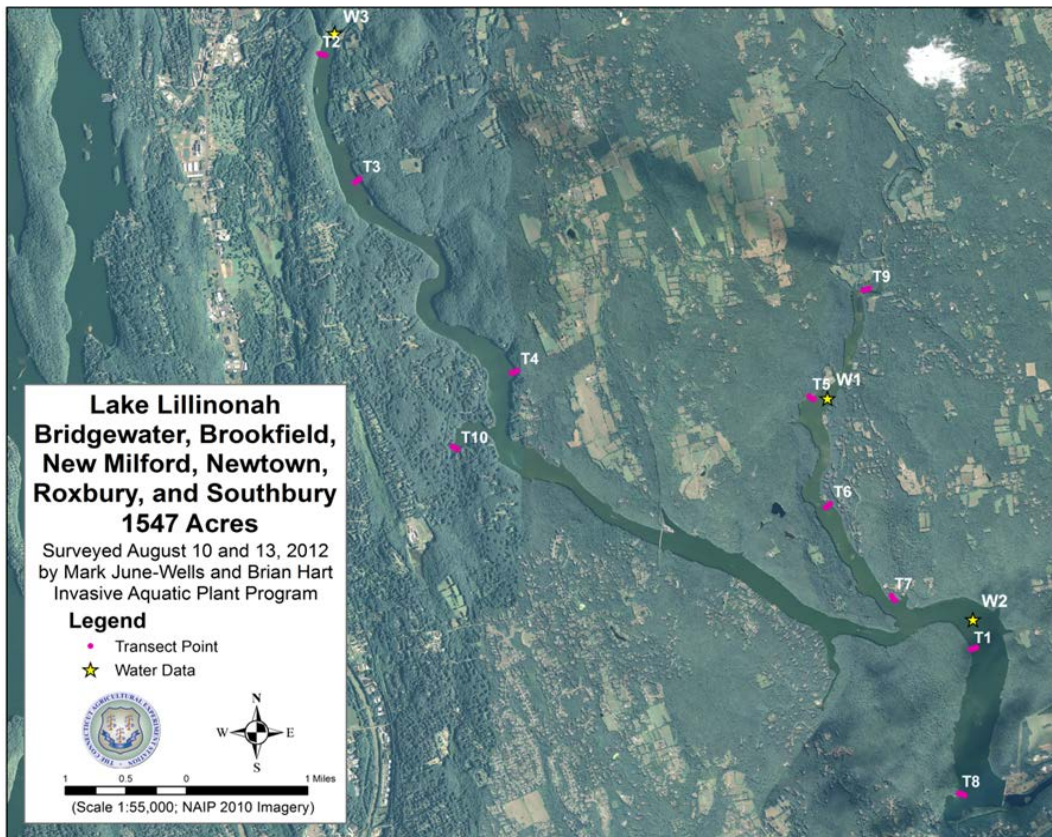
Figure 13. Locations of transects and water sampling sites in Lake Lillinonah
