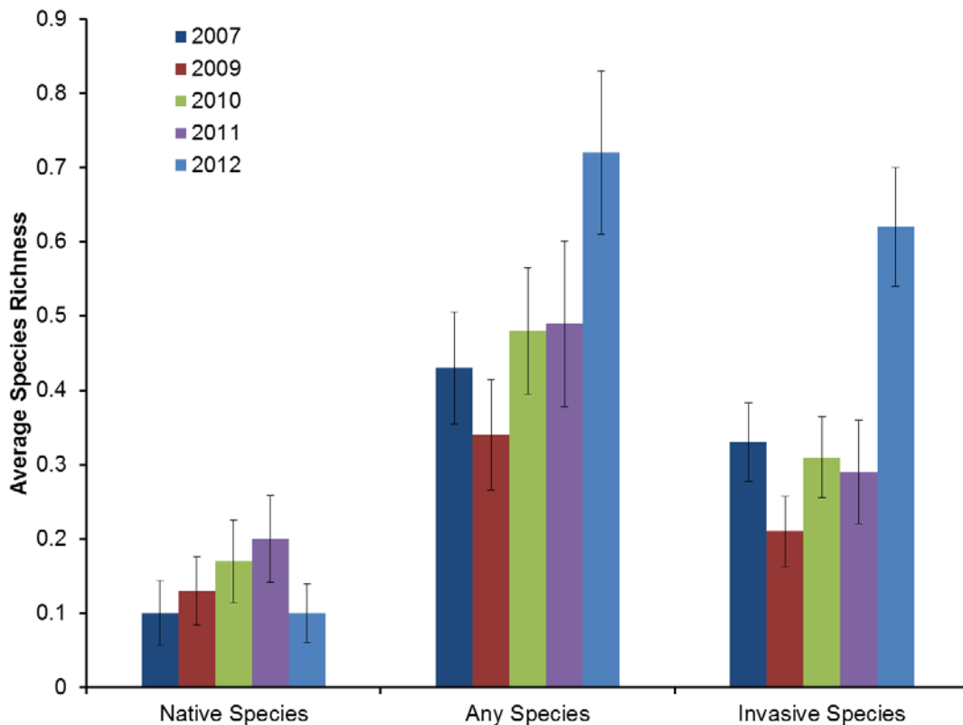
Figure 12. Yearly comparisons of the average number of species per transect point in Lake Lillinonah. Error bars equal +/- one standard error of the mean.
