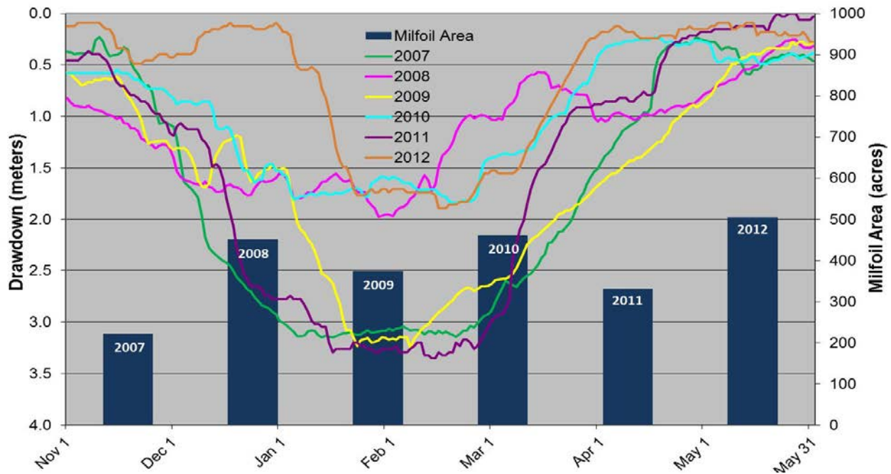
Figure 6. Yearly comparisons of drawdown depth and duration with milfoil area.
