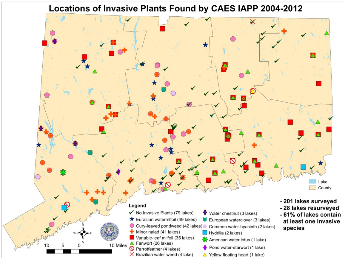
Figure 1. Locations of invasive aquatic plants found by CAES IAPP from 2004 – 2012.
