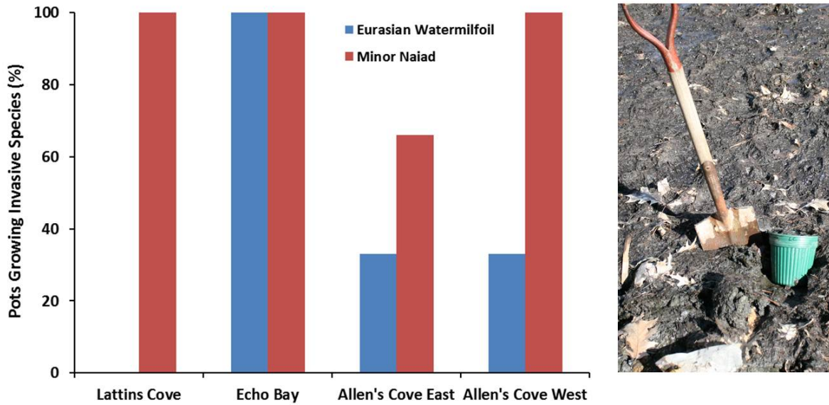
Figure 11. Growth of invasive aquatic plants (left) in sediment obtained after drawdown (right).
