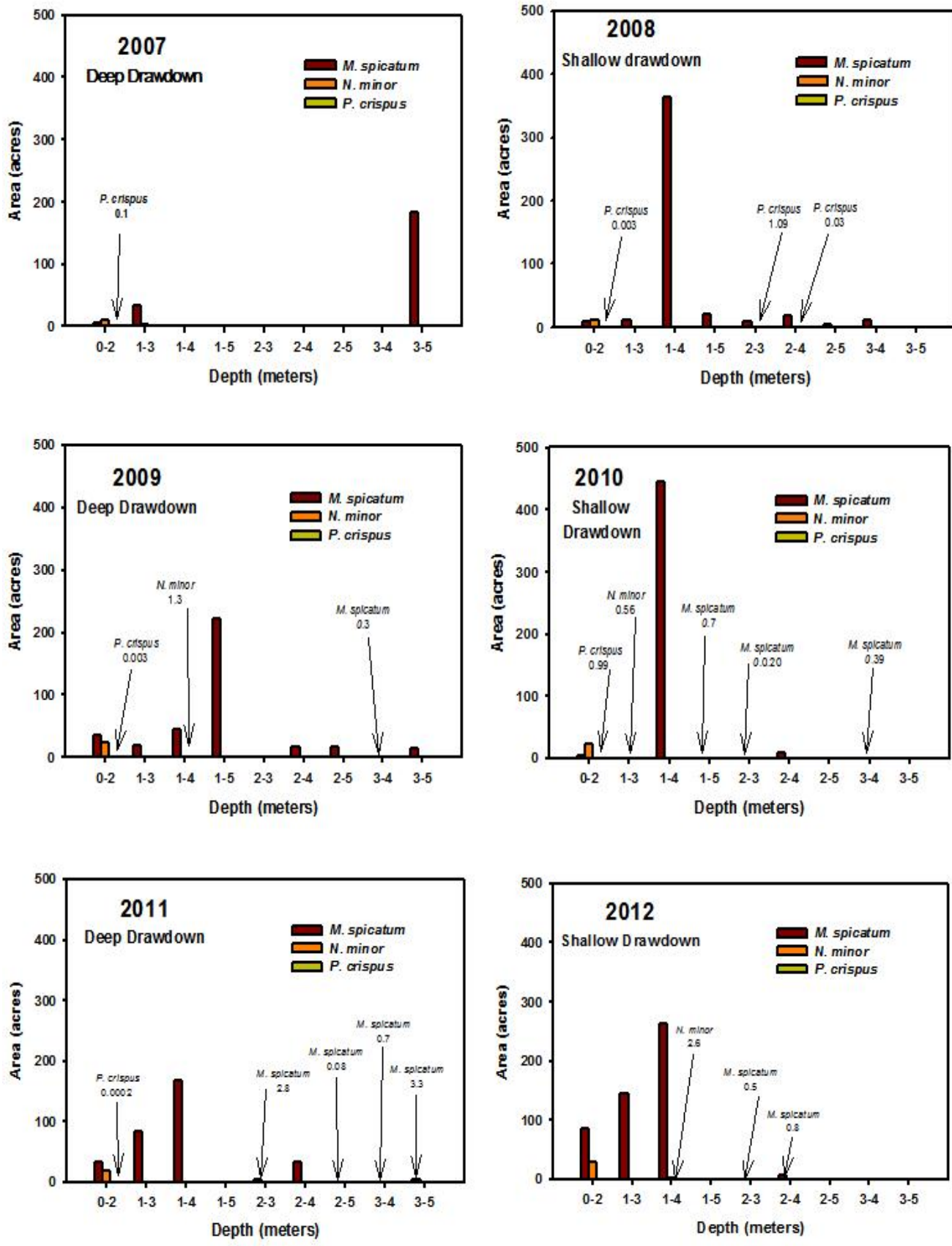
Figure 3. Yearly comparisons of depth preferences of invasive plants in Candlewood Lake.
