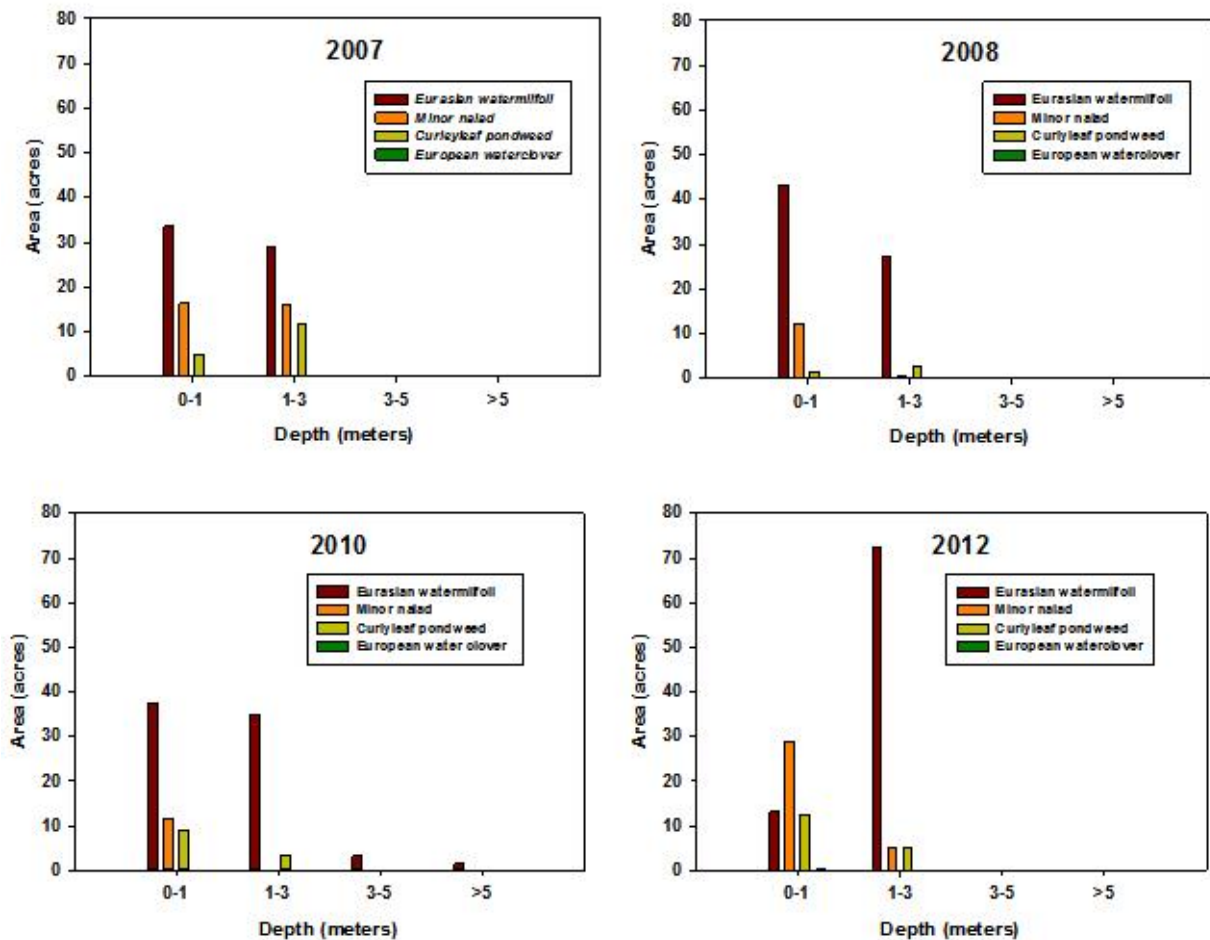
Figure 15. Yearly comparisons of the depth preferences of invasive plants in Lake Zoar.
